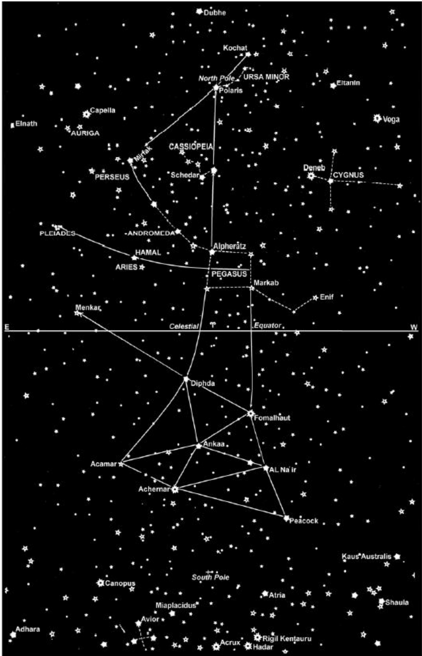
Figure 1533. Stars in the vicinity of Pegasus.
