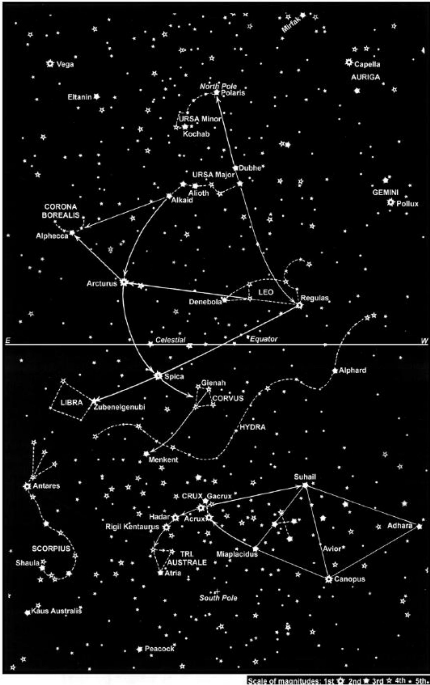
Figure 1535. Stars in the vicinity of Ursa Major.
