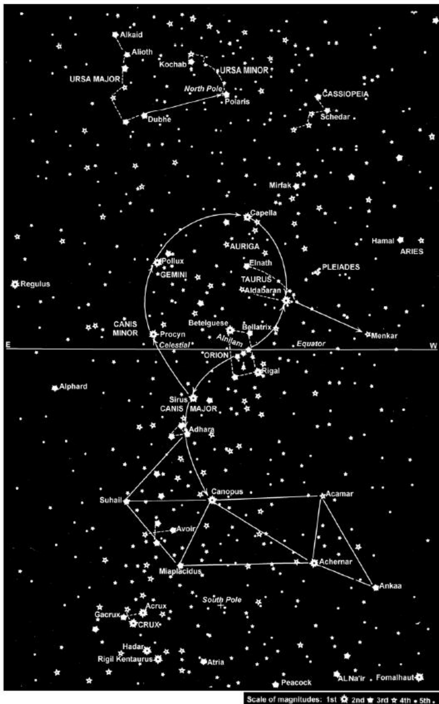
Figure 1534. Stars in the vicinity of Orion.
